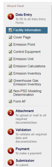
Figure 14 Wizard Panel
